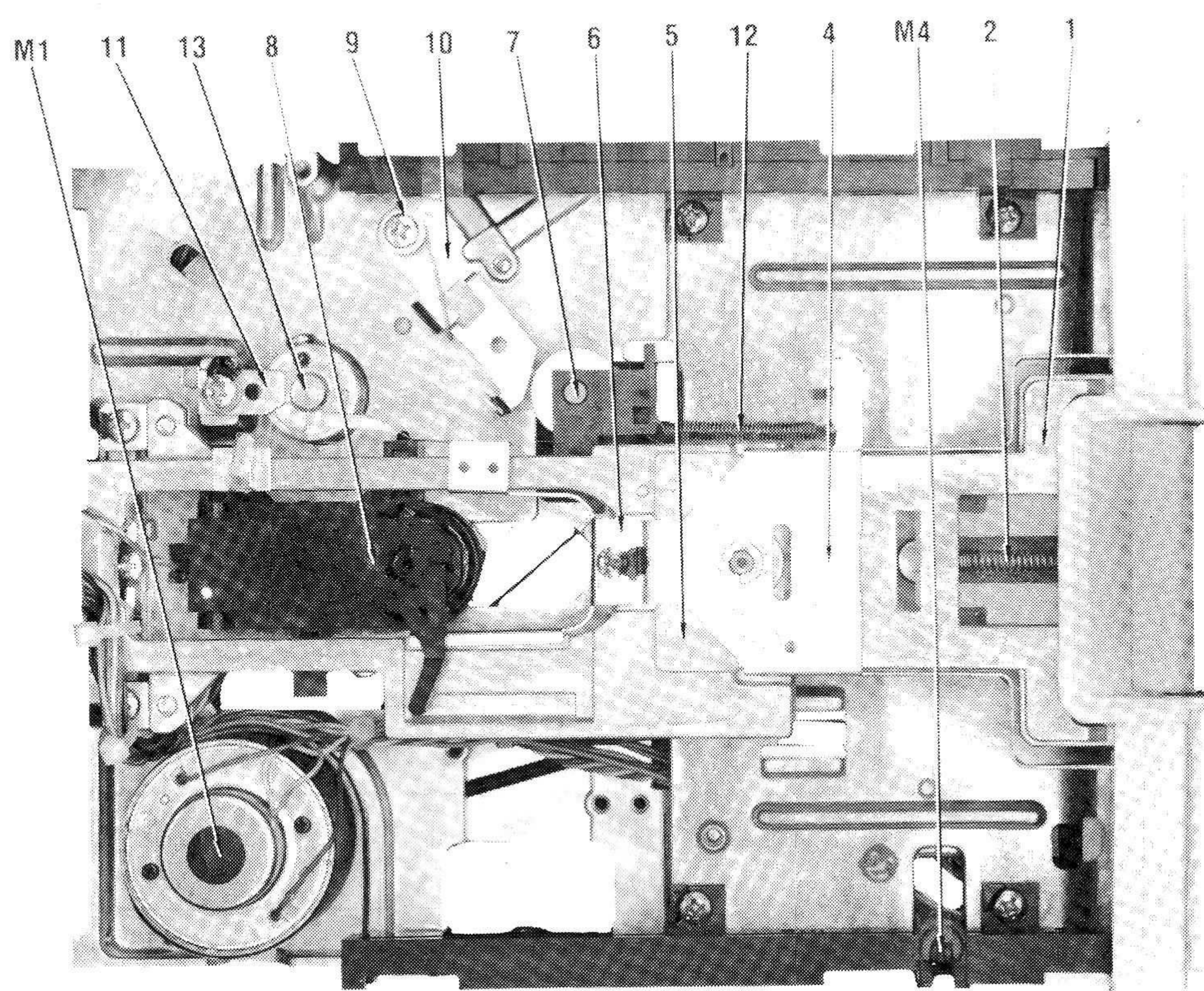
MECHANICAL-TOP VIEW
