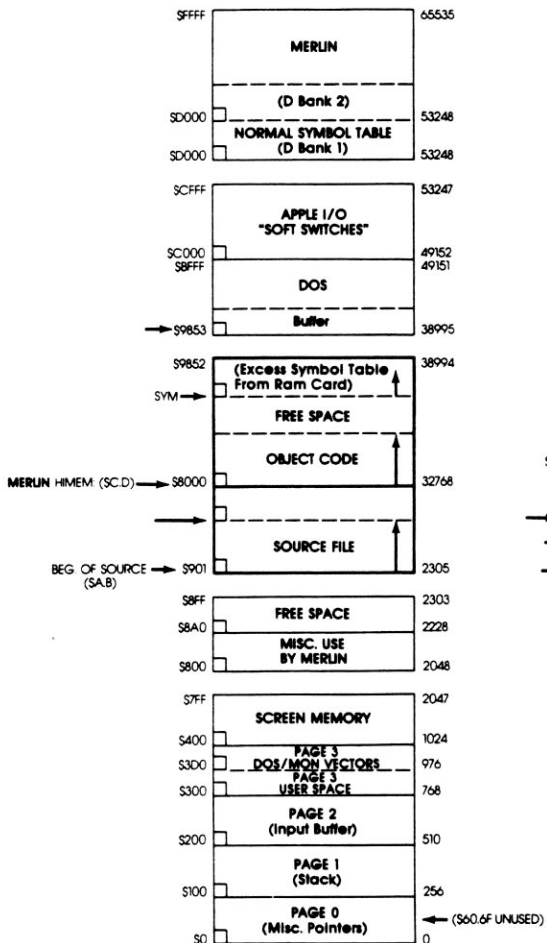
MEMORY MAP MERLIN ONLY (RAM CARD VERSION)
