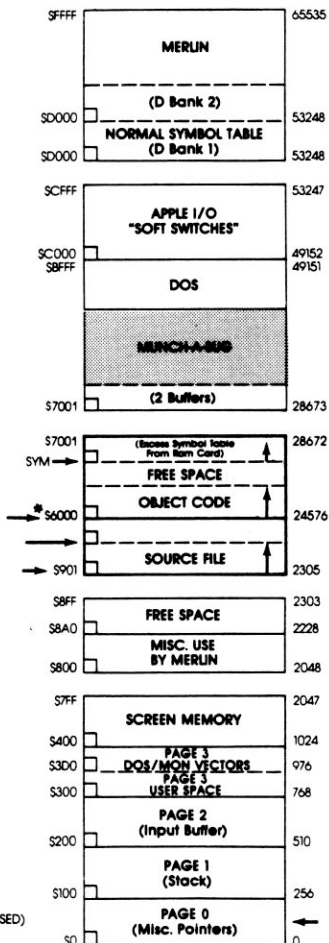
MEMORY MAP MERLIN + MAB (RAM CARD VERSION)
