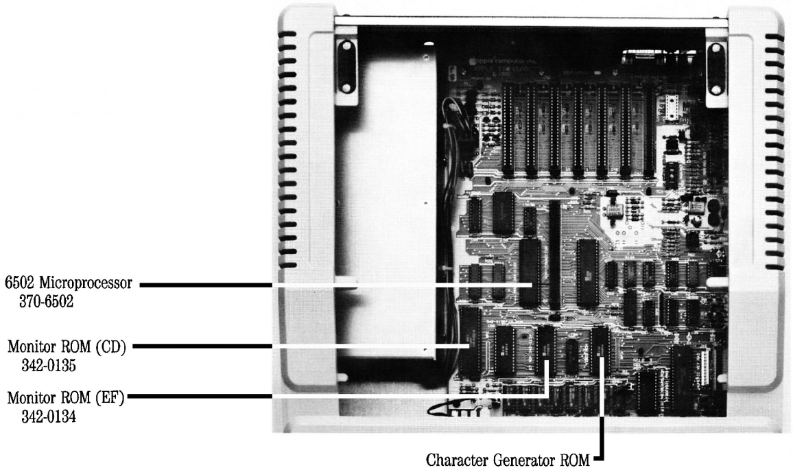
Figure 2. Chips on European (PAL) Main Logic Board
