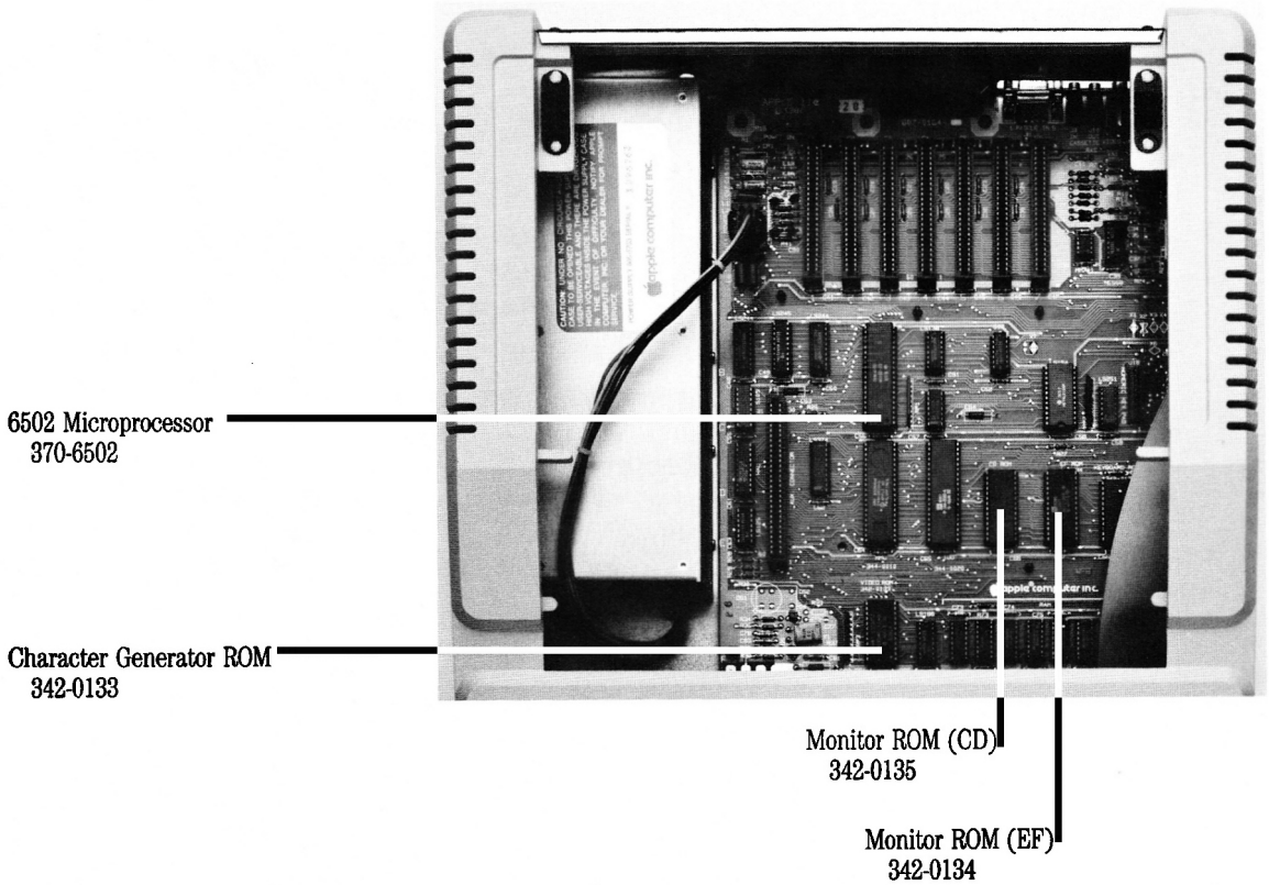
Figure 1. Chips on U.S. (NTSC) Main Logic Board
