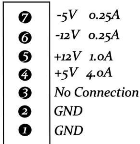
Apple IIGS Motherboard Power Connector
