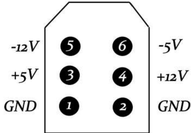
Apple II+ IIe Power Socket
