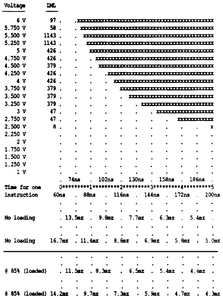
Figure 1: Typical Shmoo Plot
