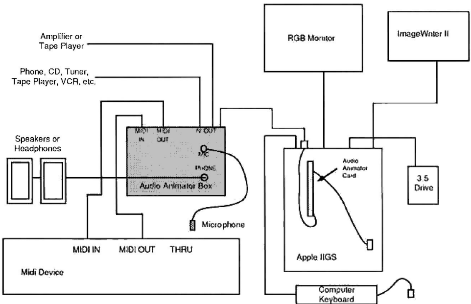
Typical Setup
