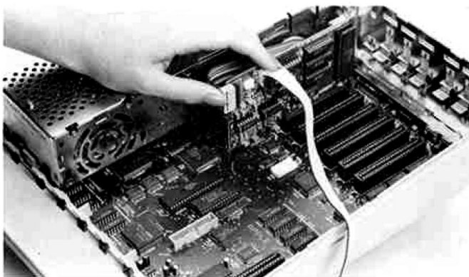
Attach 15-pin connector to card
